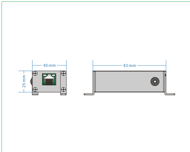
FS-RJ45/PoE-1000
